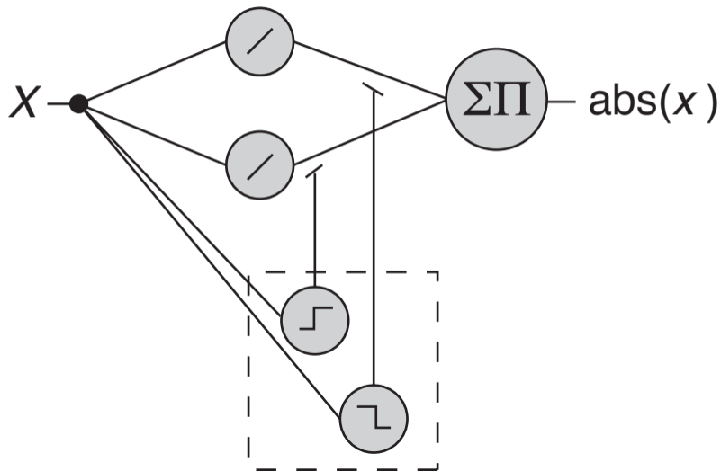
B. Mixture of expert for absolute function
