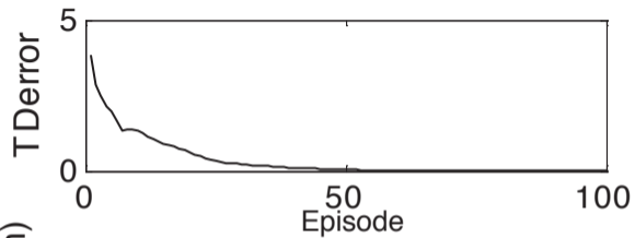
B. Temporal difference rule ( \gamma = 0.8 )
