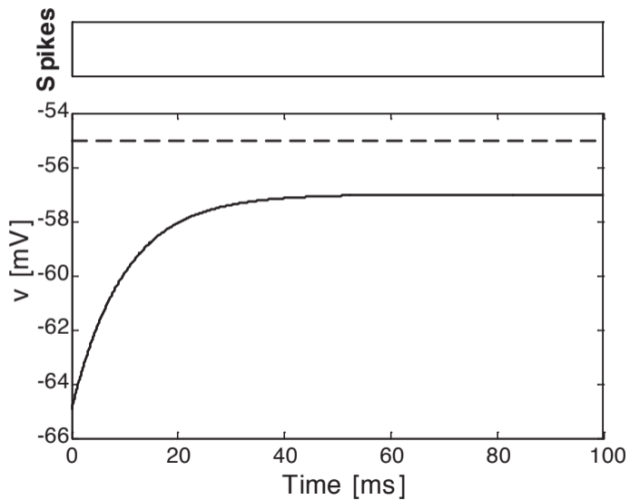
A. External input R I_{\text{ext}} = 8 \text{ mV} < \text{threshold}
