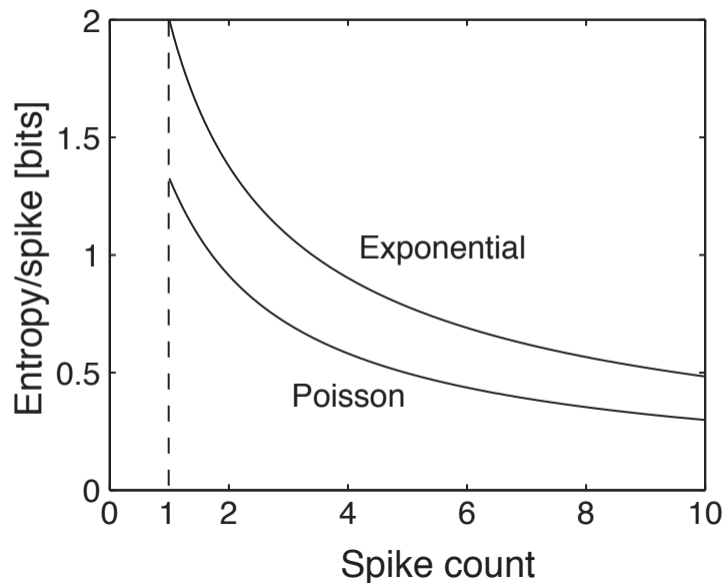
B. Maximum entropy with rate code
