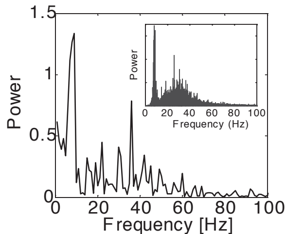
B. Power spectrum in random network
