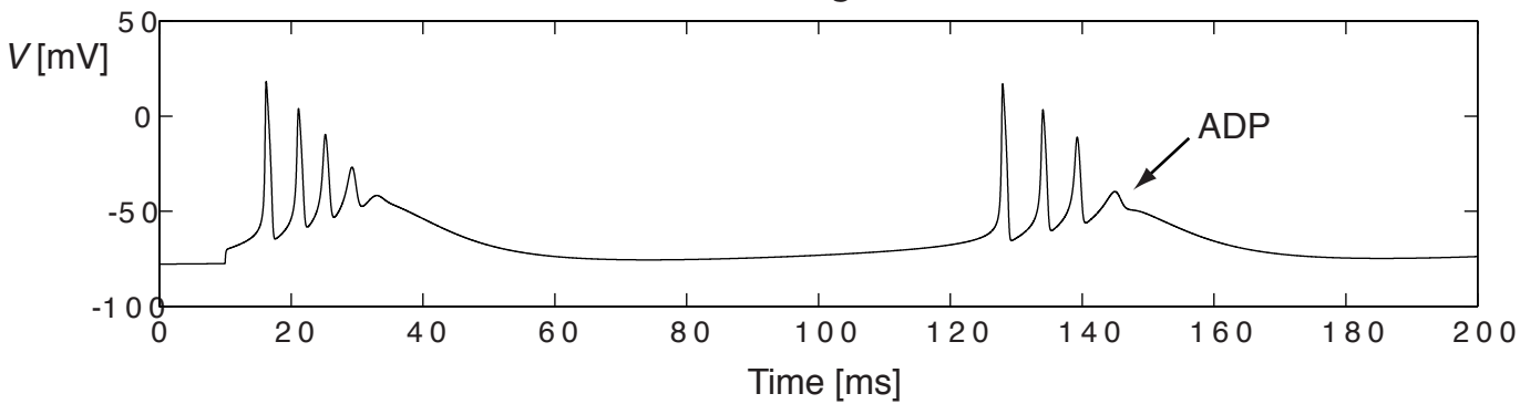
C. Bursting neuron
