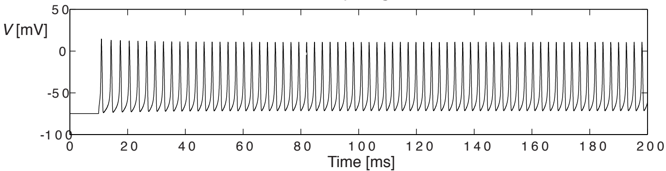
B. Regular spiking neuron
