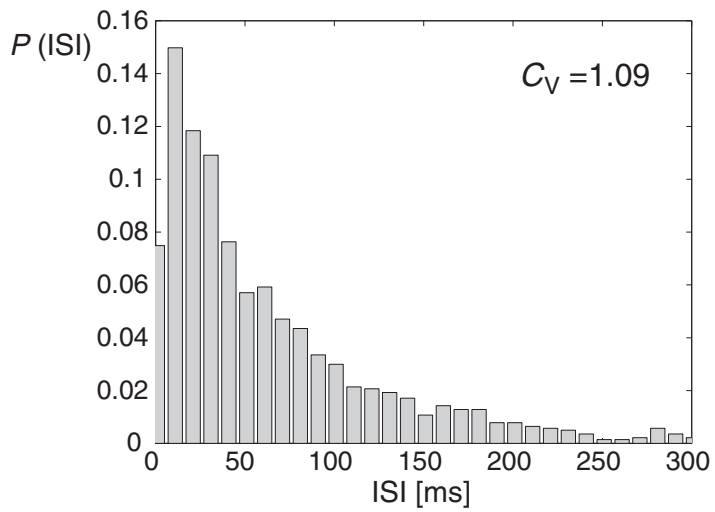
A. ISI-histogram from cell data
