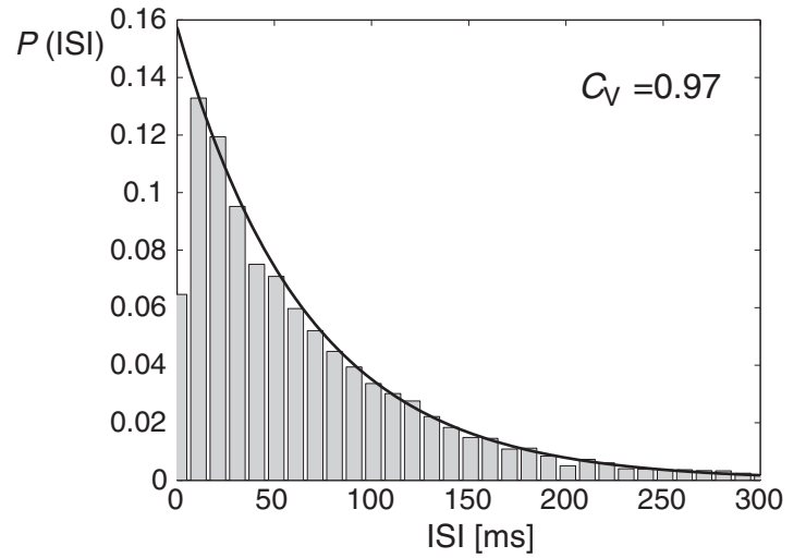
B. ISI-histogram from Poisson spike train
