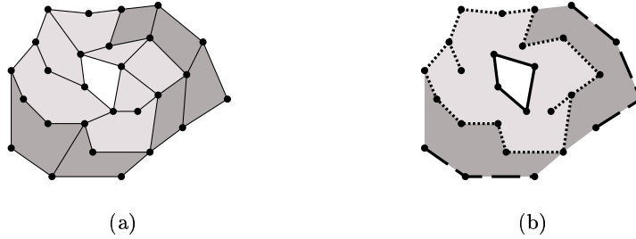
Fig. 5. (a) A graph G with its faces colored according to their levels; level 0 white, level 1 light grey, level 2 dark grey. (b) H_0 (solid), H_1 (dotted), H_2 (dashed).
