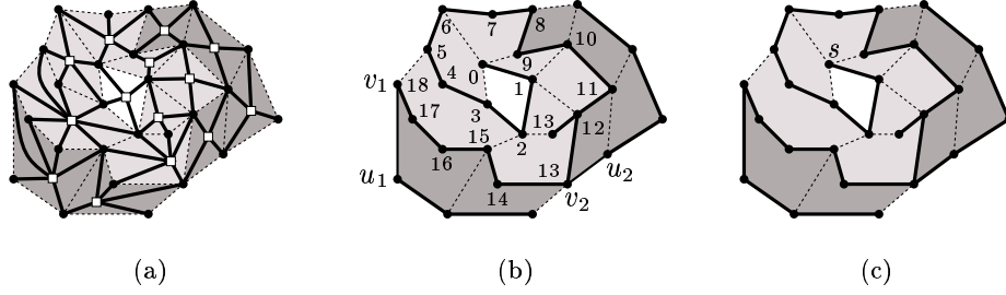
Fig. 6. (a) G^\dagger shown in bold. (b) T_1 , H_2 and attachment edges \{u_i, v_i\} . Vertices in T_1 are labeled with their DFS-depths. (c) The DFS tree.
