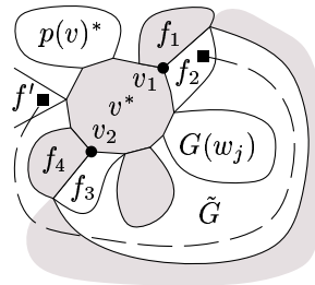
Fig. 4. Grey regions are in H_\sigma(i) .
