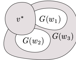
Fig. 3. The boundary of v^* \cup G(w_3) is not a simple cycle.
