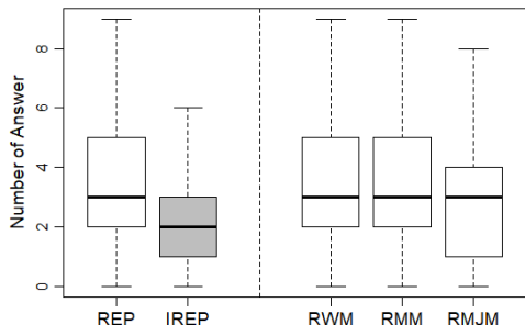
Fig. 13: Number of answers for the questions with reproducible and irreproducible issues
