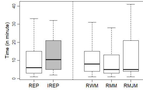
Fig. 11: Time spent for reproducible and irreproducible issues
