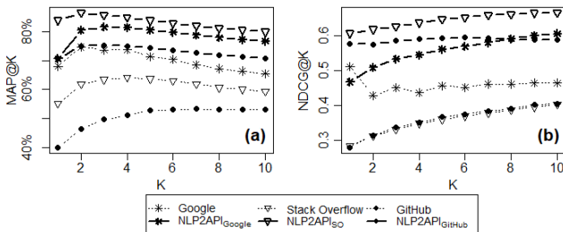
Fig. 7. Comparison between popular web/code search engines and NLP2API in relevant code segment retrieval using (a) MAP@K and (b) NDCG@K
