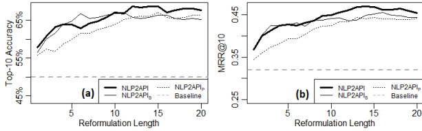
Fig. 6. Reformulated vs. baseline query using (a) Top-10 accuracy and (b) MRR@10
