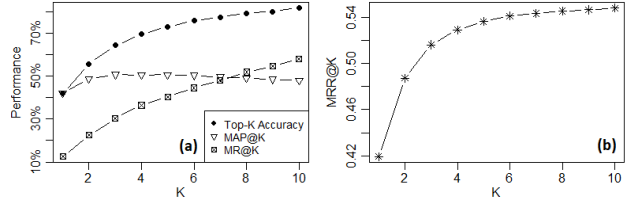
Fig. 3. Performance of NLP2API in API class suggestion for various Top-K results
