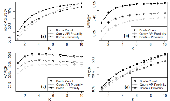
Fig. 5. Comparison between Borda count and Query-API proximity in estimating API relevance using (a) accuracy, (b) reciprocal rank, (c) precision, and (d) recall
