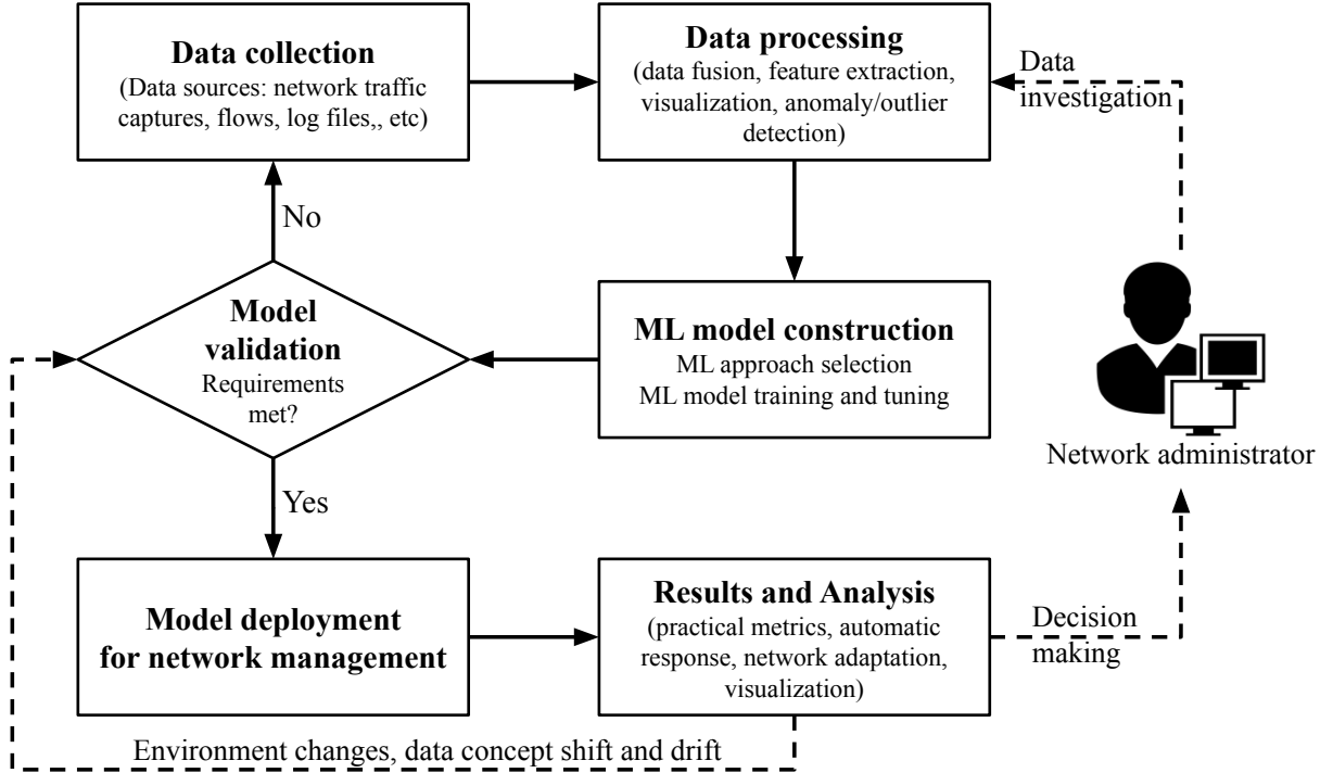
Fig. 1 A ML workflow in network/system management (adapted with changes from [4])
