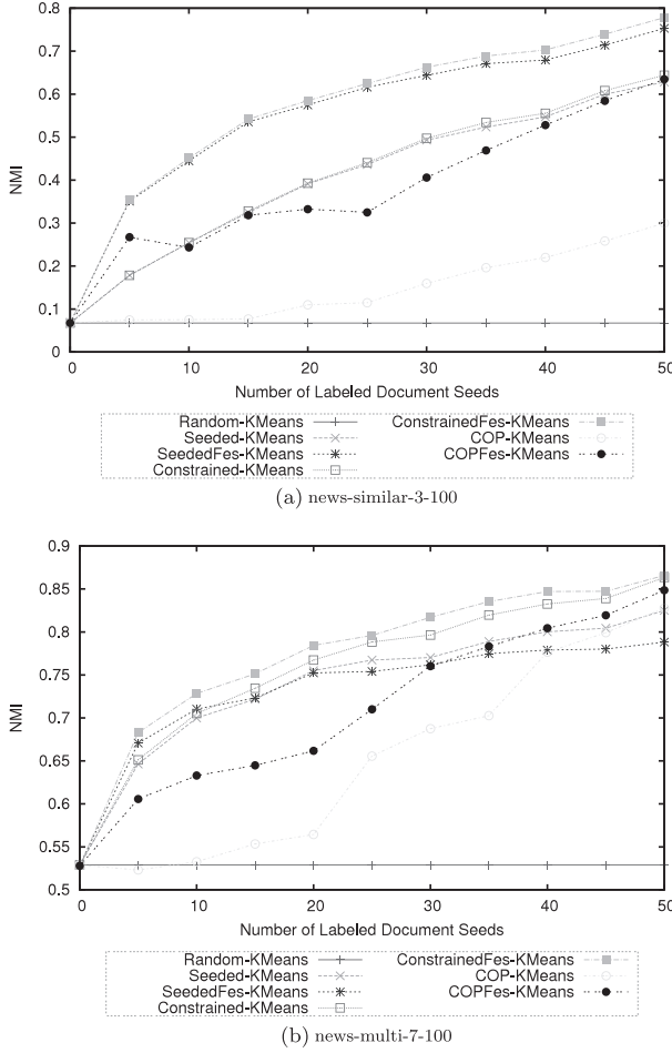
FIGURE 10. Different numbers of document seeds (constraints for COP K -means and COPFes K -means are generated from document seeds; refer to Section 5.4 for details). (a) news-similar-3-100 and (b) news-multi-7-100. NMI, normalized mutual information.
