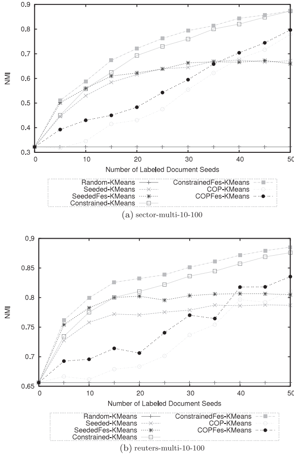
FIGURE 12. Different numbers of document seeds (constraints for COP K -means and COPFes K -means are generated from document seeds; refer to Section 5.4 for details). (a) sector-multi-10-100 and (b) reuters-multi-10-100. NMI, normalized mutual information.
