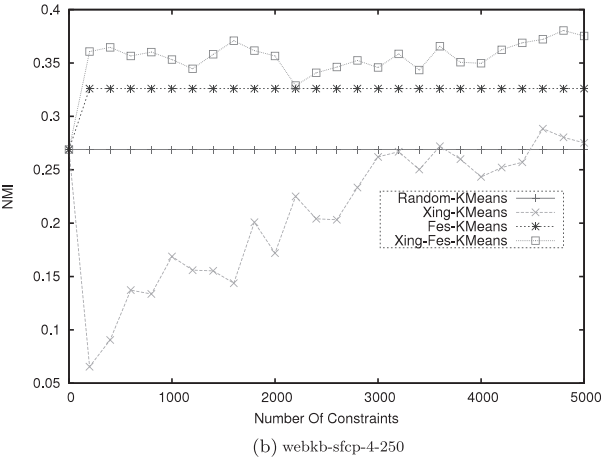
FIGURE 13. Metric learning method and feature supervision method. (a) sector-multi-10-100 and (b) webkb-sfcp-4-250. NMI, normalized mutual information.
