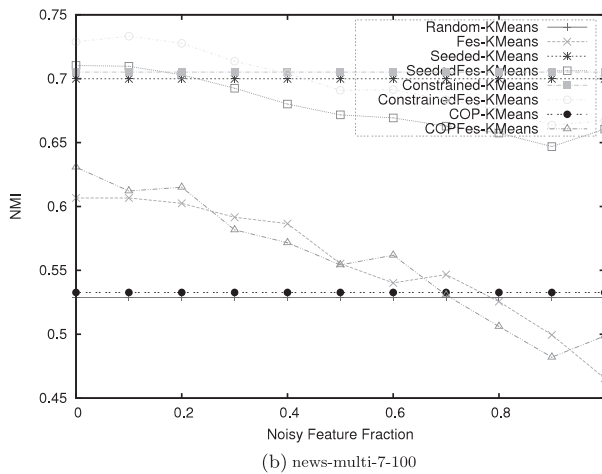
FIGURE 8. Enhanced with feature supervision with varying noise feature fractions. (a) sector-multi-10-100 and (b) news-multi-7-100. NMI, normalized mutual information.
