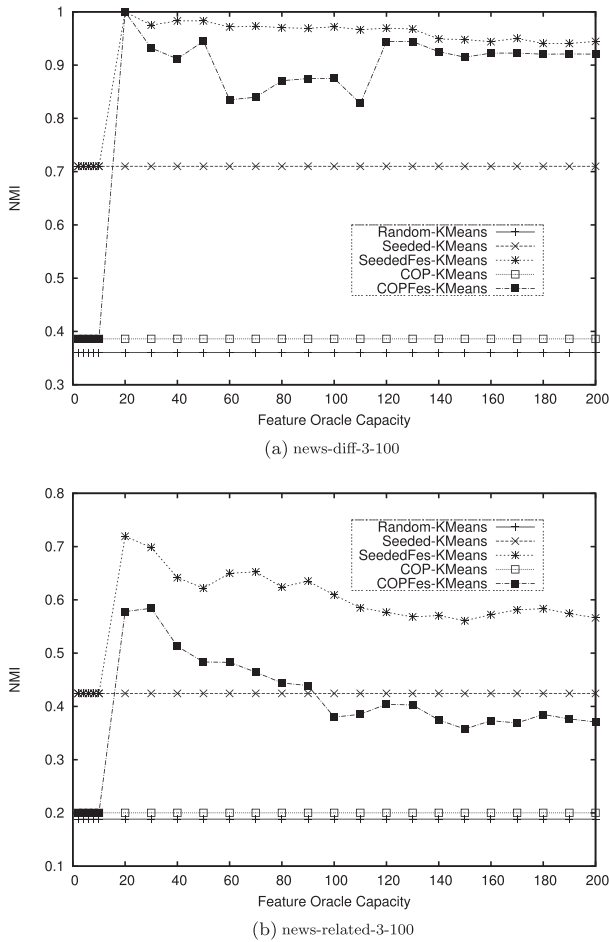
FIGURE 3. Performance as a function of the size of feature vocabulary, i.e., feature oracle capacity. (a) news-diff-3-100 and (b) news-related-3-100. NMI, normalized mutual information.
