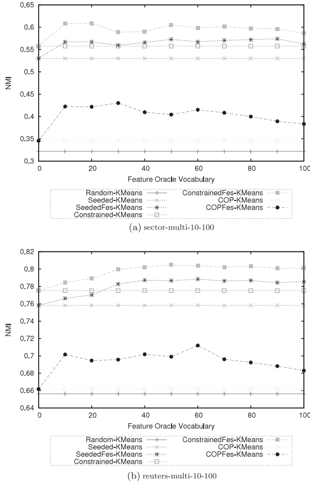
FIGURE 6. Performance as a function of the size of feature vocabulary, i.e., feature oracle capacity. (a) sector-multi-10-100 and (b) reuters-multi-10-100. NMI, normalized mutual information.
