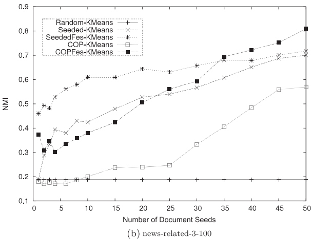
(b) news-related-3-100
