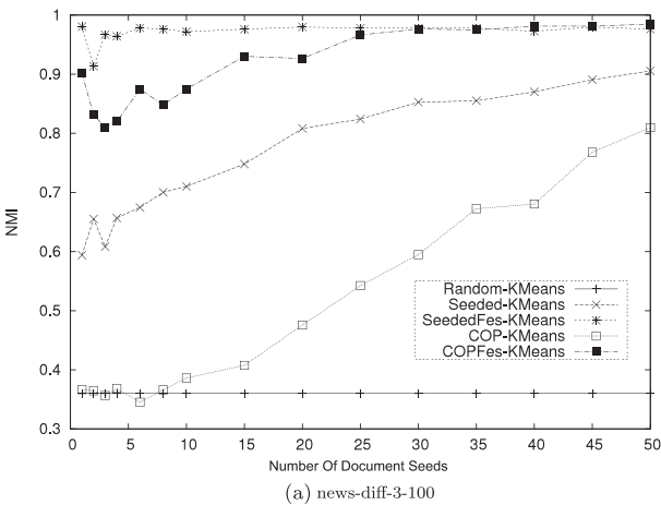
(a) news-diff-3-100
