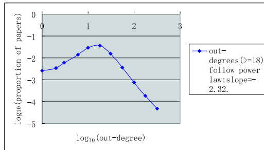
Fig. 4. The out-degree distribution in the union citation graph
