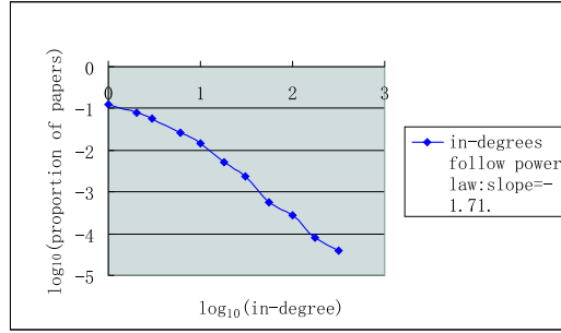
Fig. 3. The in-degree distribution in the union citation graph in computer science literature subscribe to the power law with exponent=1.71.
