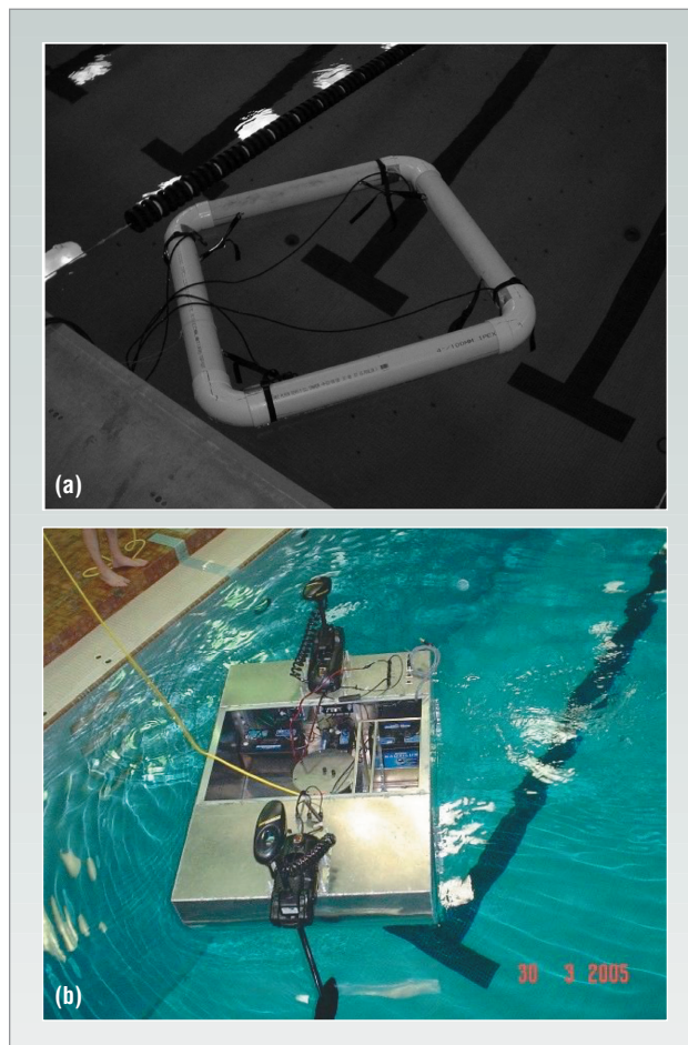
Figure 5. Surface-based sensing. (a) The passive acoustic raft with four omnidirectional hydrophones attached to a 1\text{ m} \times 1\text{ m} square buoy. (b) Self-propelled robotic surface buoy that locates itself in a surface-coordinate system and tracks the AQUA robot via a hydrophone array.
