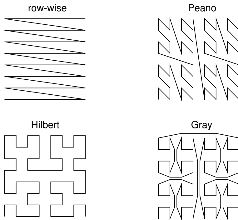
Figure C.8: Common space filling curves.
