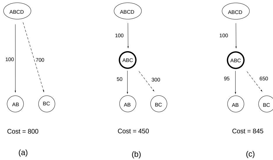
Figure 4.11: Pruning ineffective nodes. Case (a) shows the original tree. In case (b), a more dense ABC node offers great benefit. However, in case (c), we see that a sparse ABC node actually increase the cost.
