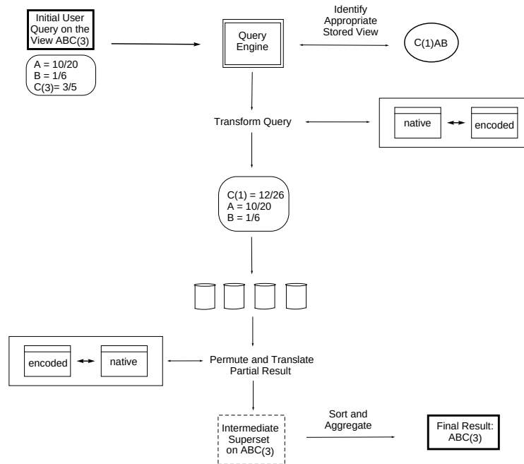
Figure 5.12: The process of resolving a user query containing a hierarchical attribute.
