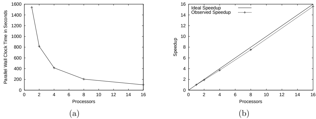
Figure 5.13: (a) Parallel wall clock time for index construction, and (b) the corresponding Speedup.
