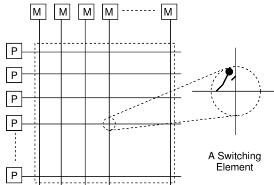
Figure A.4: A crossbar switch.
