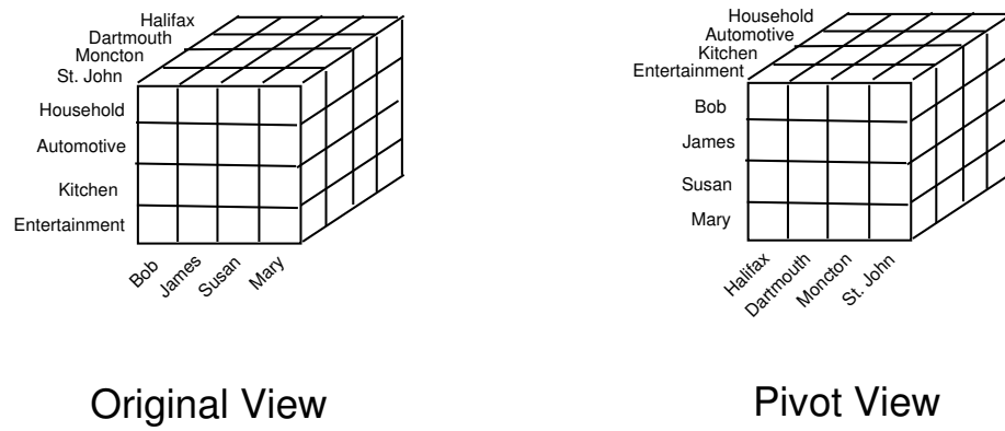
Figure 2.4: The Pivot operation.
