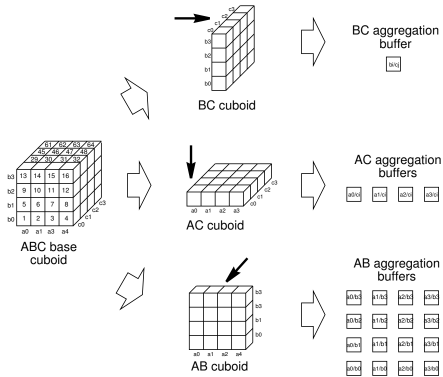
Figure 2.14: Generating group-bys with ArrayCube.
