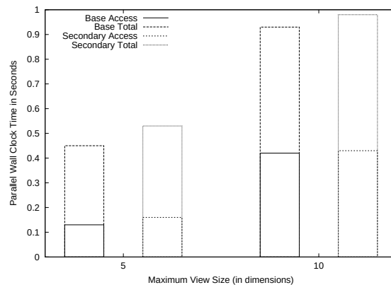
Figure 5.20: Querying performance using hierarchical attributes.
