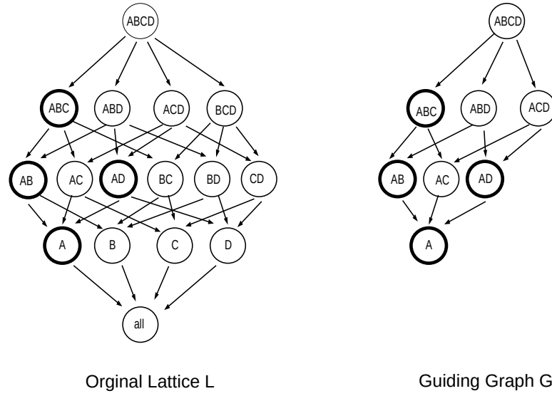
Figure 4.5: Graph Pruning, where bolded views belong to the selected set S .
