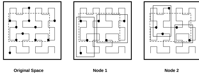
Figure 5.4: Striping the data across two nodes. (Block capacity = 3)
