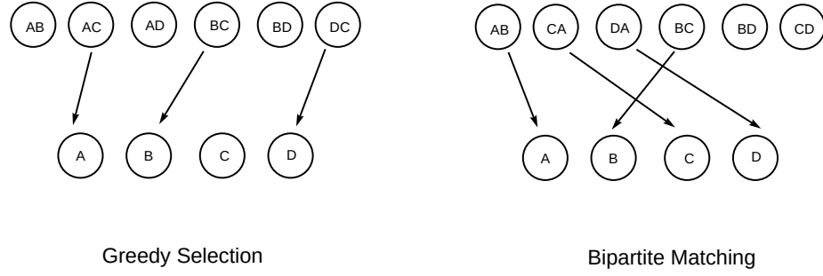
Figure 4.8: An example of how the greedy algorithm might identify fewer scan edges than the bipartite matching approach. In this case, the greedy method did not produce a scan edge for C .
