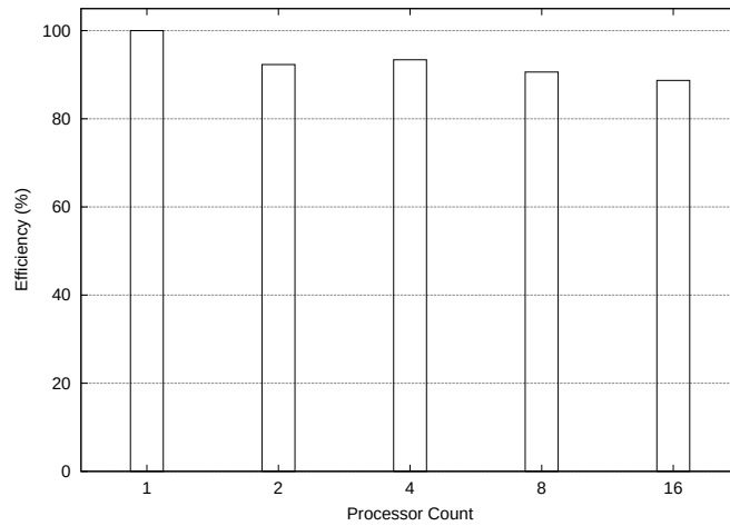
Figure 4.20: Efficiency ratings when considering “build” times only.
