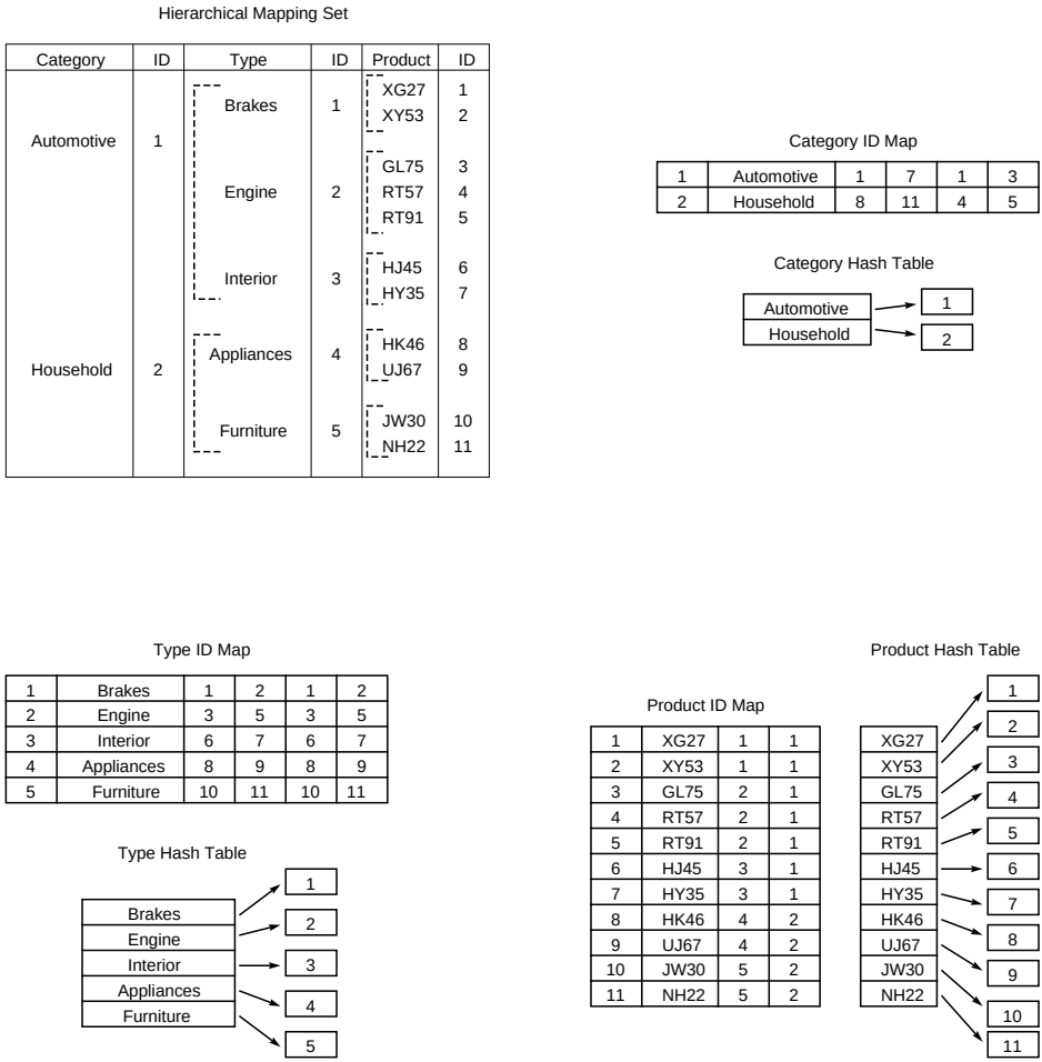
Figure 5.11: The mapping tables.
