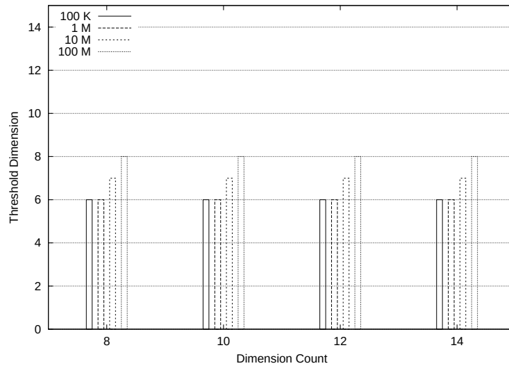
Figure 5.7: The density threshold for varying dimension counts and data set sizes. Note that a data set is considered sparse only when it contains at least 99% of the records in the original fact table.
