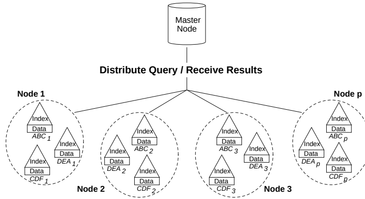
Figure 5.2: The distributed data cube R-tree model.
