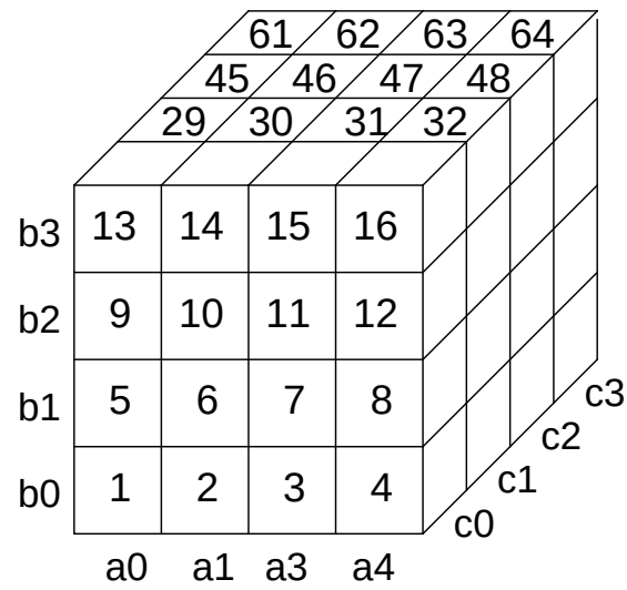
Figure 2.12: A three-dimensional chunked cube.
