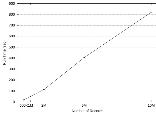
Figure 3.9: Record count evaluation.
