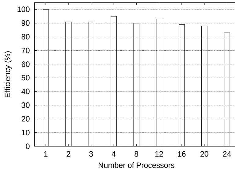
Figure 3.6: Efficiency ratings for the Linux cluster.
