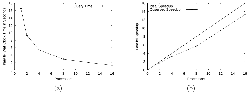
Figure 5.14: (a) Wall clock time for distributed query resolution, and (b) the corresponding Speedup.
