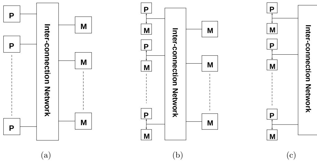
Figure A.2: (a) All memory is global. (b) Processors have a mix of local and global memory. (c) All memory is local. Hardware provides remote memory access.
