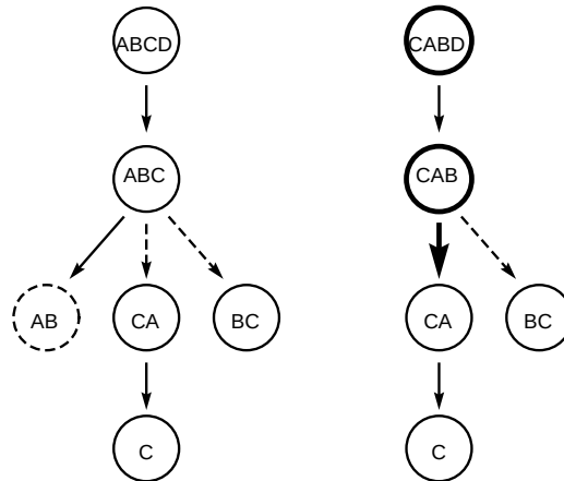
Figure 4.7: Illustration of FixPipelines ( R ). The dashed view is not included in the reduced tree. The bolded nodes represent views (i) whose attributes had to be rearranged and/or (ii) were given a new scan child.
