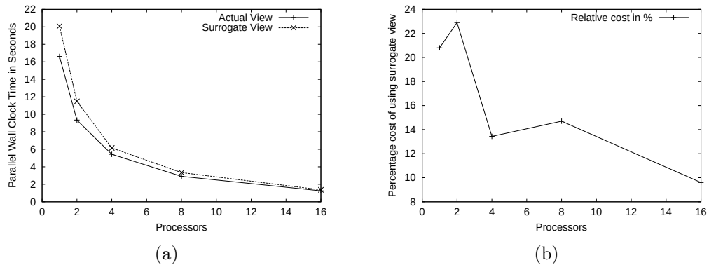
Figure 5.19: (a) Distributed query resolution in surrogate group-bys, and (b) Relative percentage cost of using surrogate view instead of materialized primary view.
