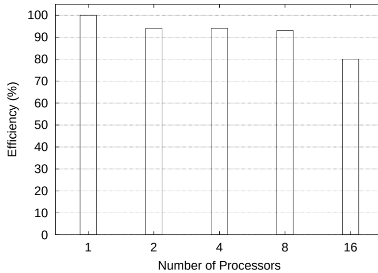
Figure 3.8: Efficiency ratings for the SunFire 6800.
