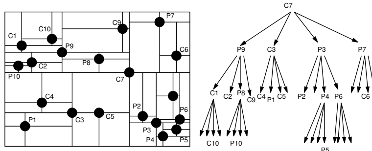
Figure C.2: The point quad-tree.
