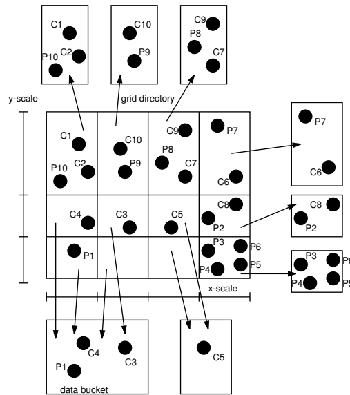
Figure C.5: The grid file.
