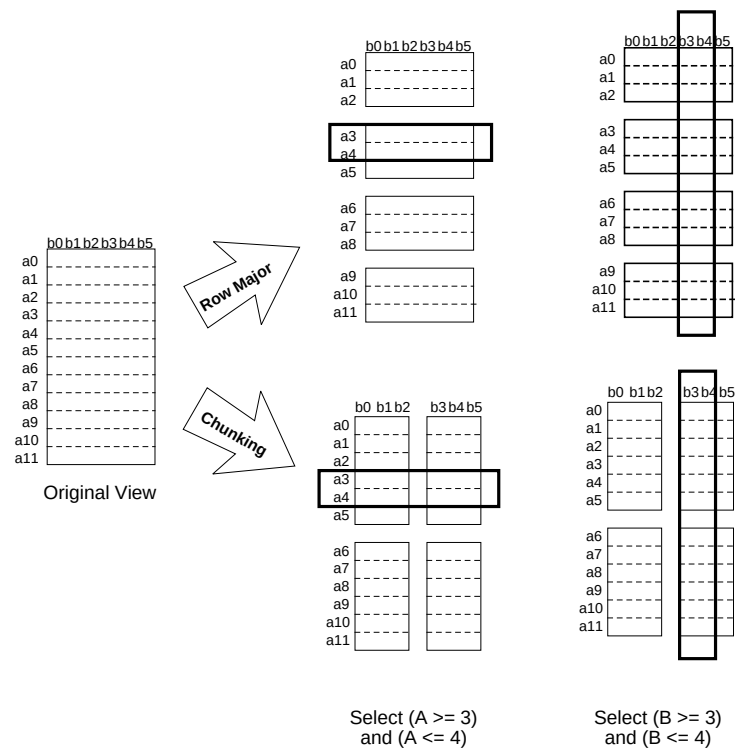
Figure 2.13: Access patterns for chunking versus row major storage.
