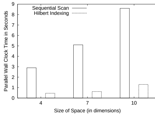
Figure 5.18: Sequential Scans versus Hilbert indexing.
