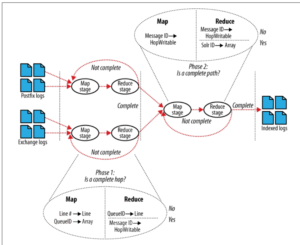
Figure 14-9. MapReduce chain
