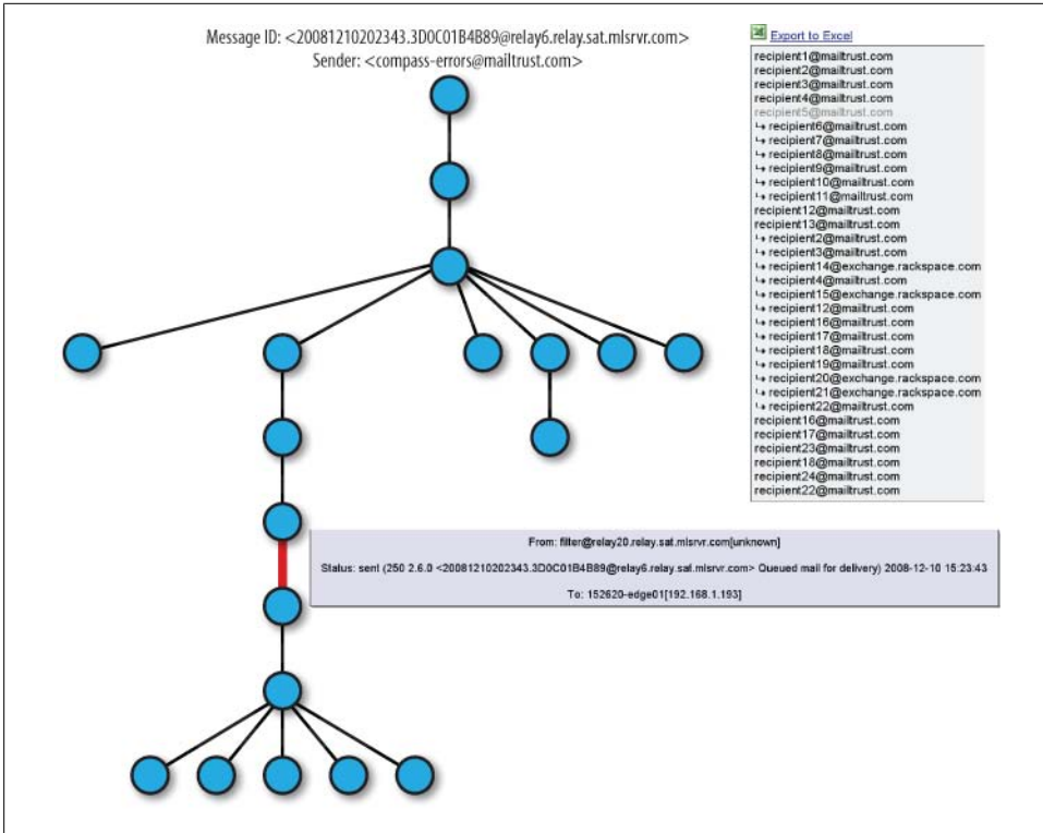
Figure 14-10. Data tree
