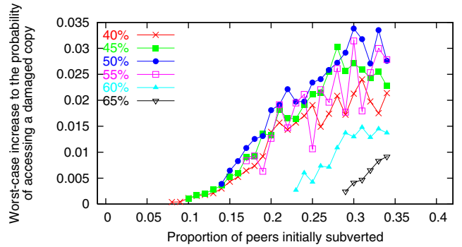
Figure 6: Worst-case increase in the probability of accessing a bad replica due to the attack, as a function of initial subversion. Each curve corresponds to runs with a different foothold ratio at the start of the attack phase, for subversions at which the adversary did not cause irrecoverable damage.
