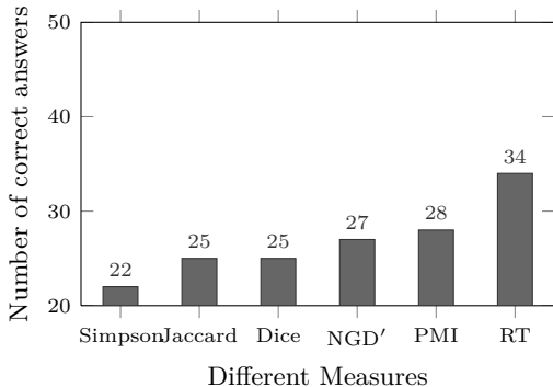
Figure 4: Results on ESL’s 50 synonym questions.
