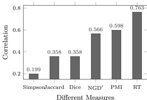
Figure 1: Similarity correlations on RG’s 65 noun pairs.
