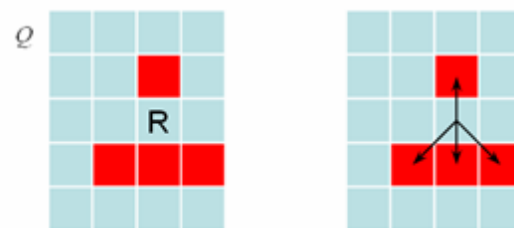
Figure 6: 180^\circ rotated edge points of Q around R (left) and four vectors of Q (right)
