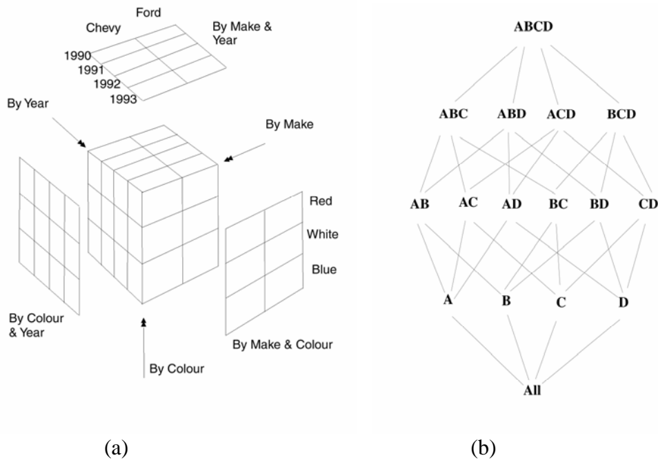
Figure 1: (a) A three dimensional datacube for automobile sales data. (b) The lattice corresponding to a four dimensional datacube with dimensions A, B, C and D.
